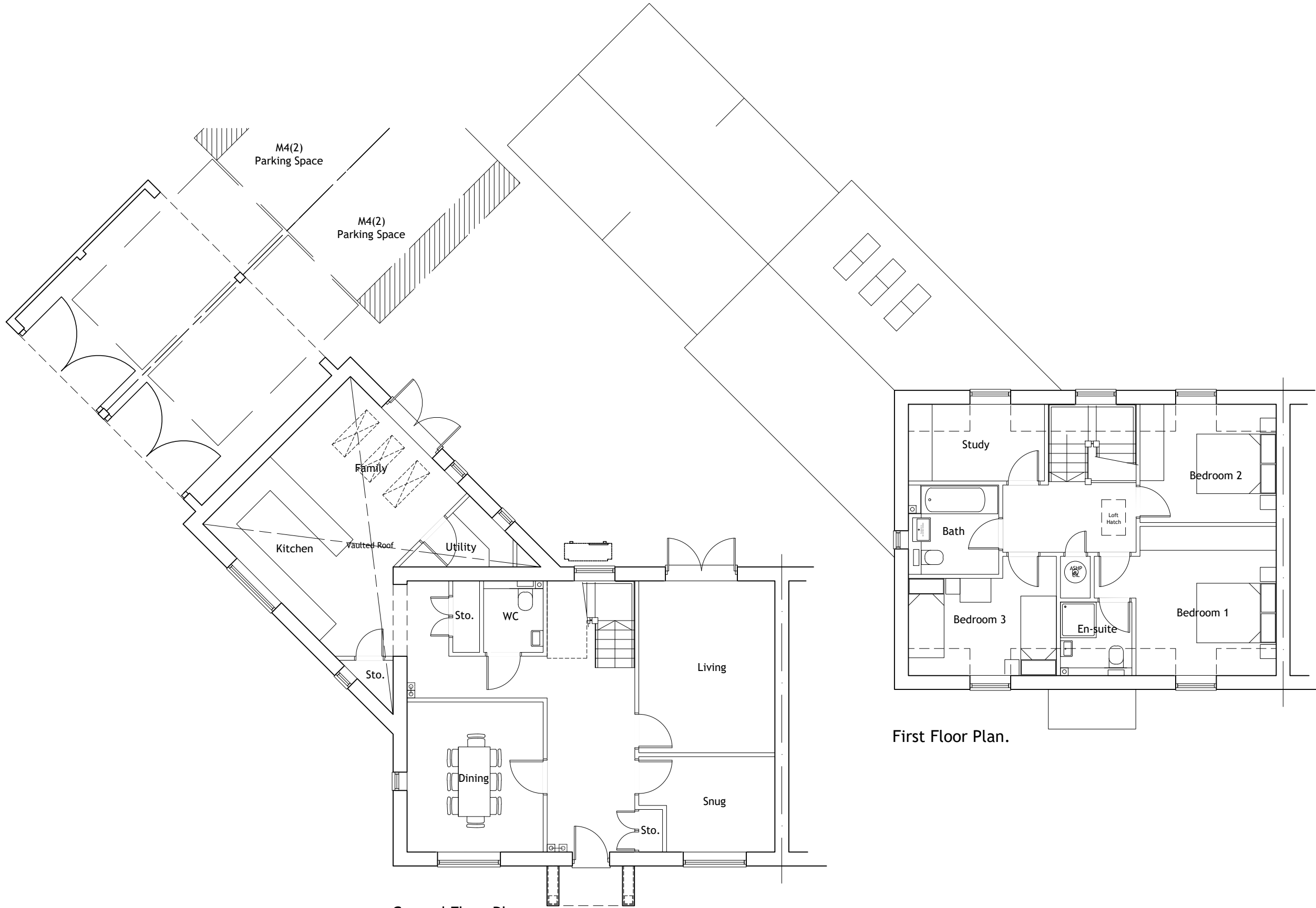
Ground Floor Plan. 155.5sq.m / 1,673sq.ft. 3 Bed 6 Person. M4(2) Compliant.
