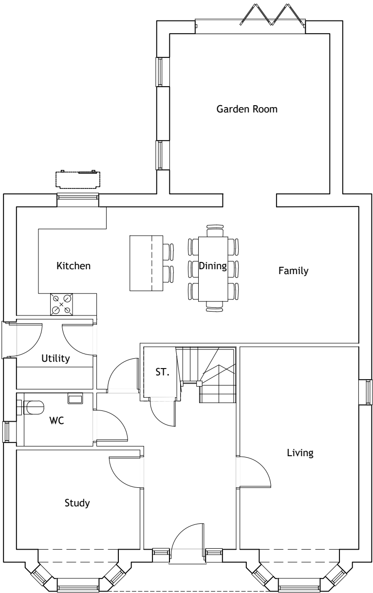
Ground Floor Plan. 215sq.m / 2,314sq.ft. 5 Bed 9 Person.
