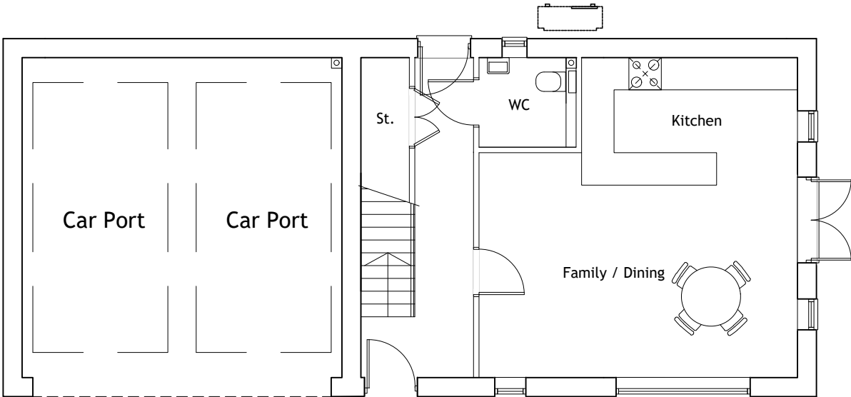
Ground Floor Plan. 109.7sq.m / 1180.8sq.ft. 2 Bed 4 Person.
