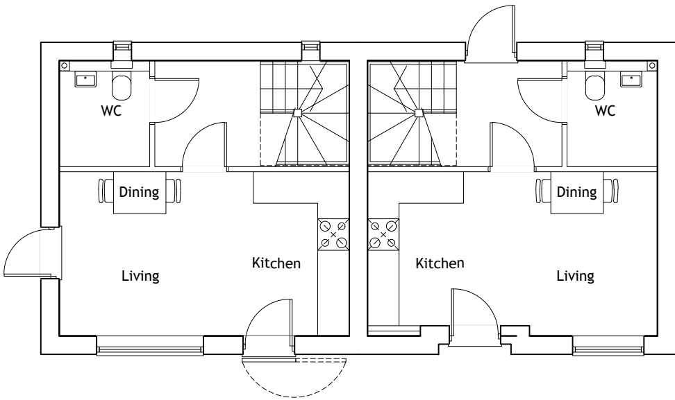
Ground Floor Plan. 58sq.m / 624sq.ft. 1 Bed 2 Person. M4(2) Compliant.
