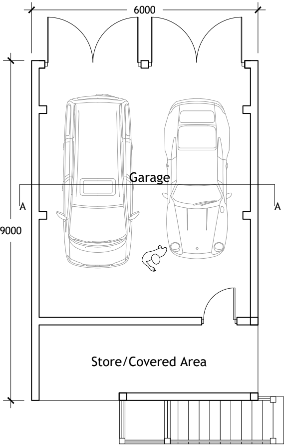
Ground Floor Plan Plot 257
