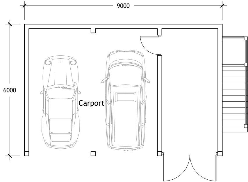
Ground Floor Plan Plots 255, 256 and 267
