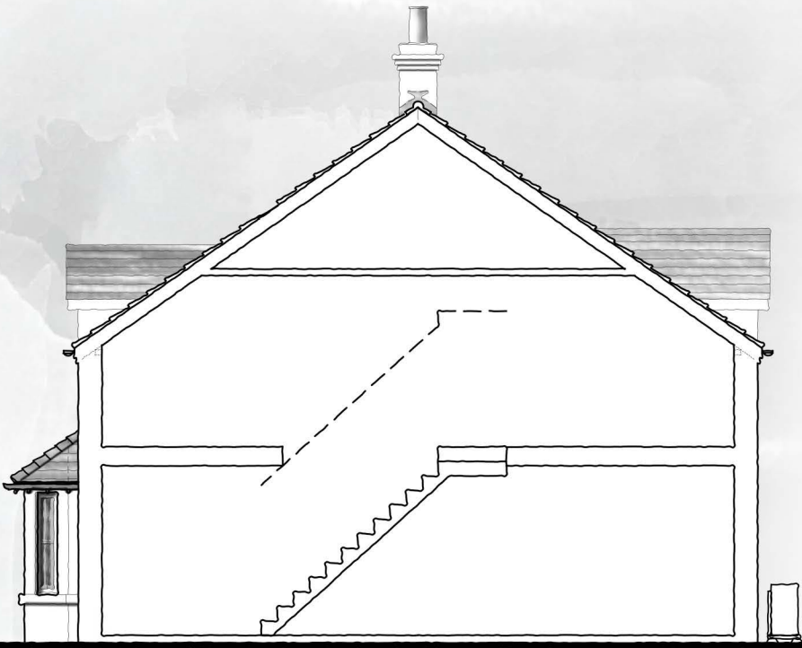
Side/Section.
